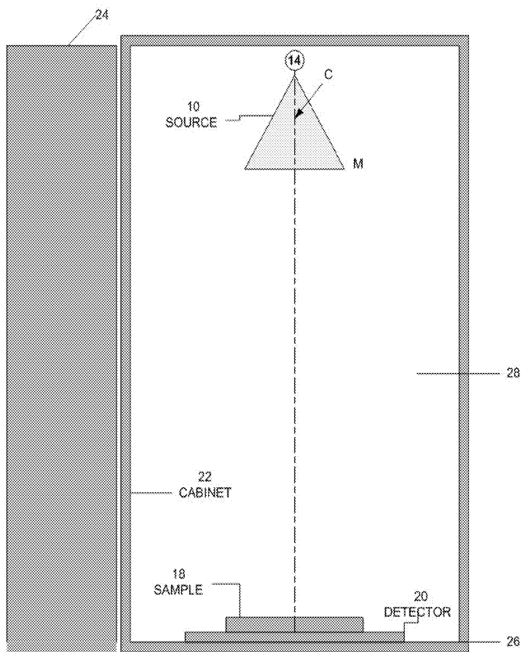
FRONT VIEW INTO CABINET Door Open Fig 2
