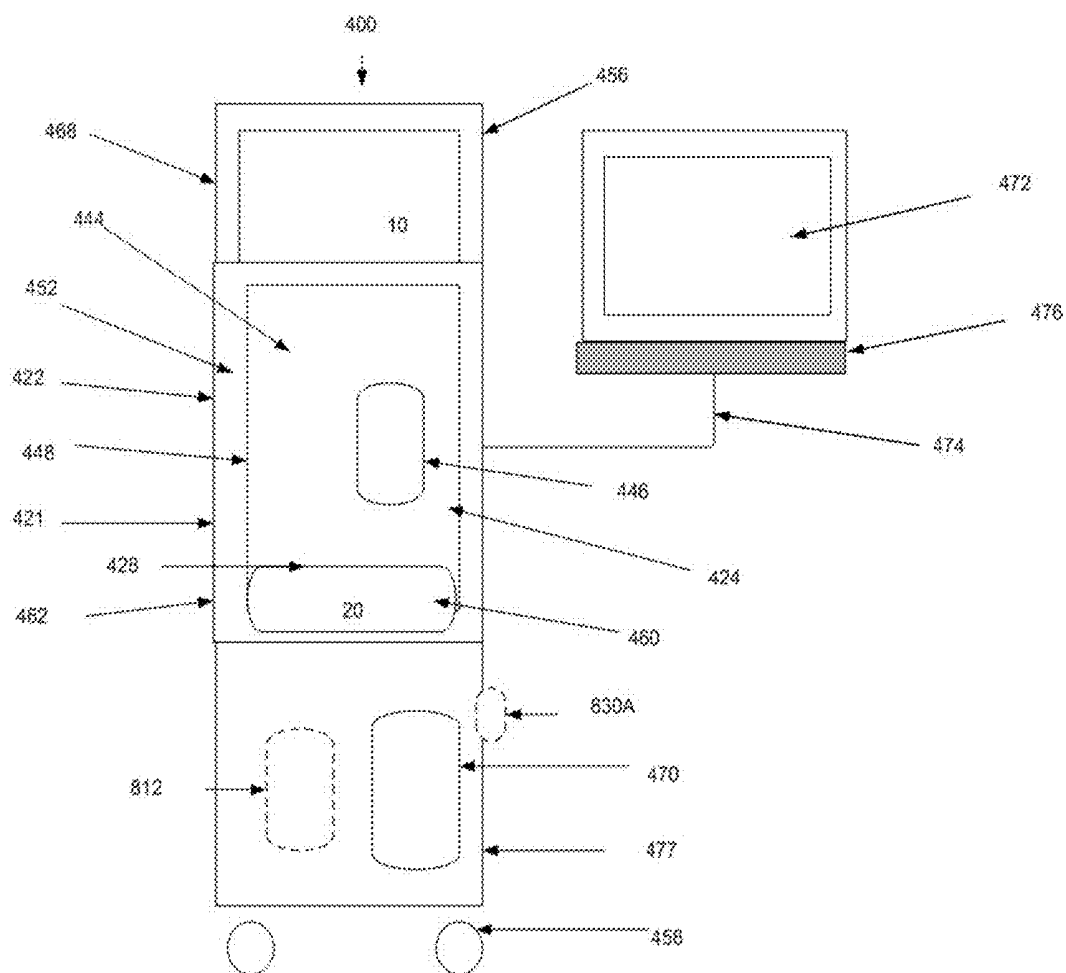
Fig. 8C – Typical Cabinet with Processor and Connection Point
