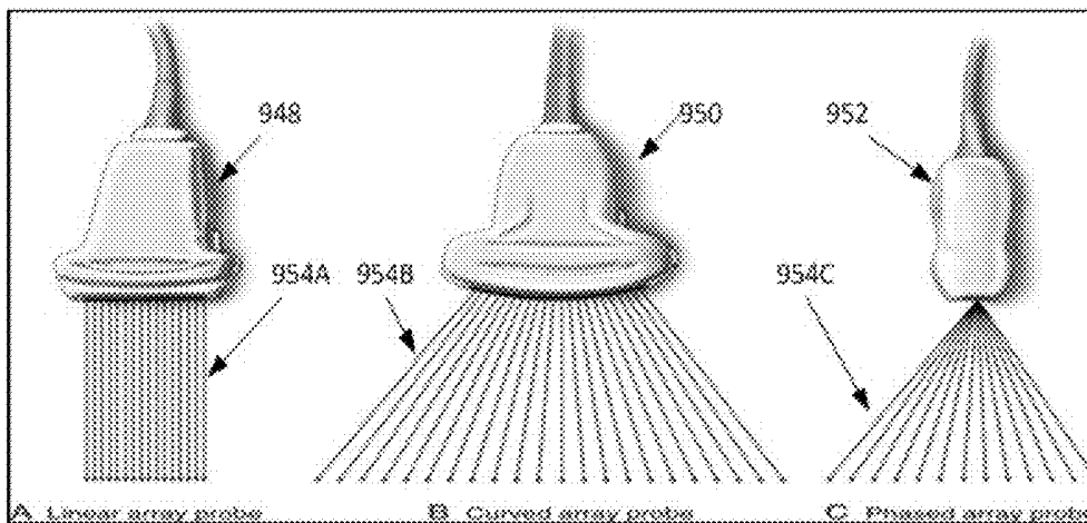
Fig. 9 – Typical Ultrasound Probes
