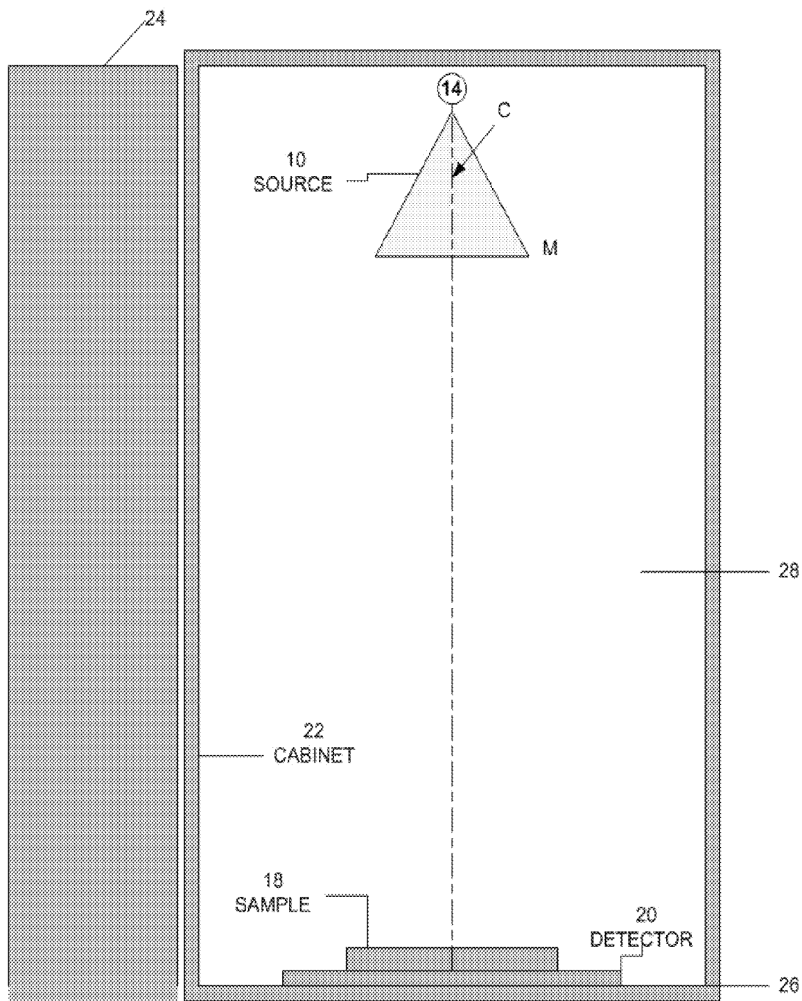
FRONT VIEW INTO CABINET
