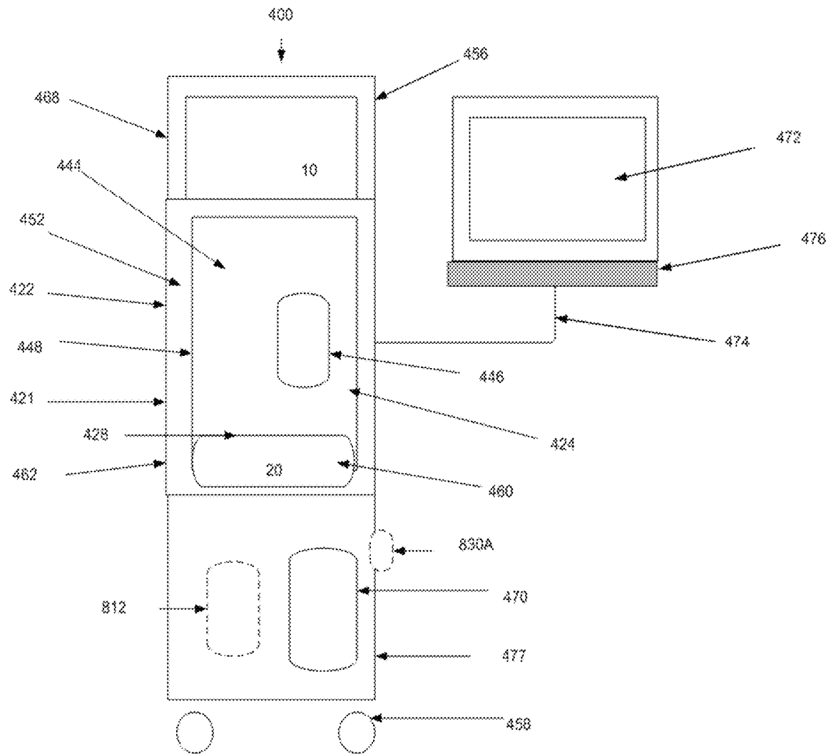
Fig. 8C – Typical Cabinet with Processor and Connection Point
