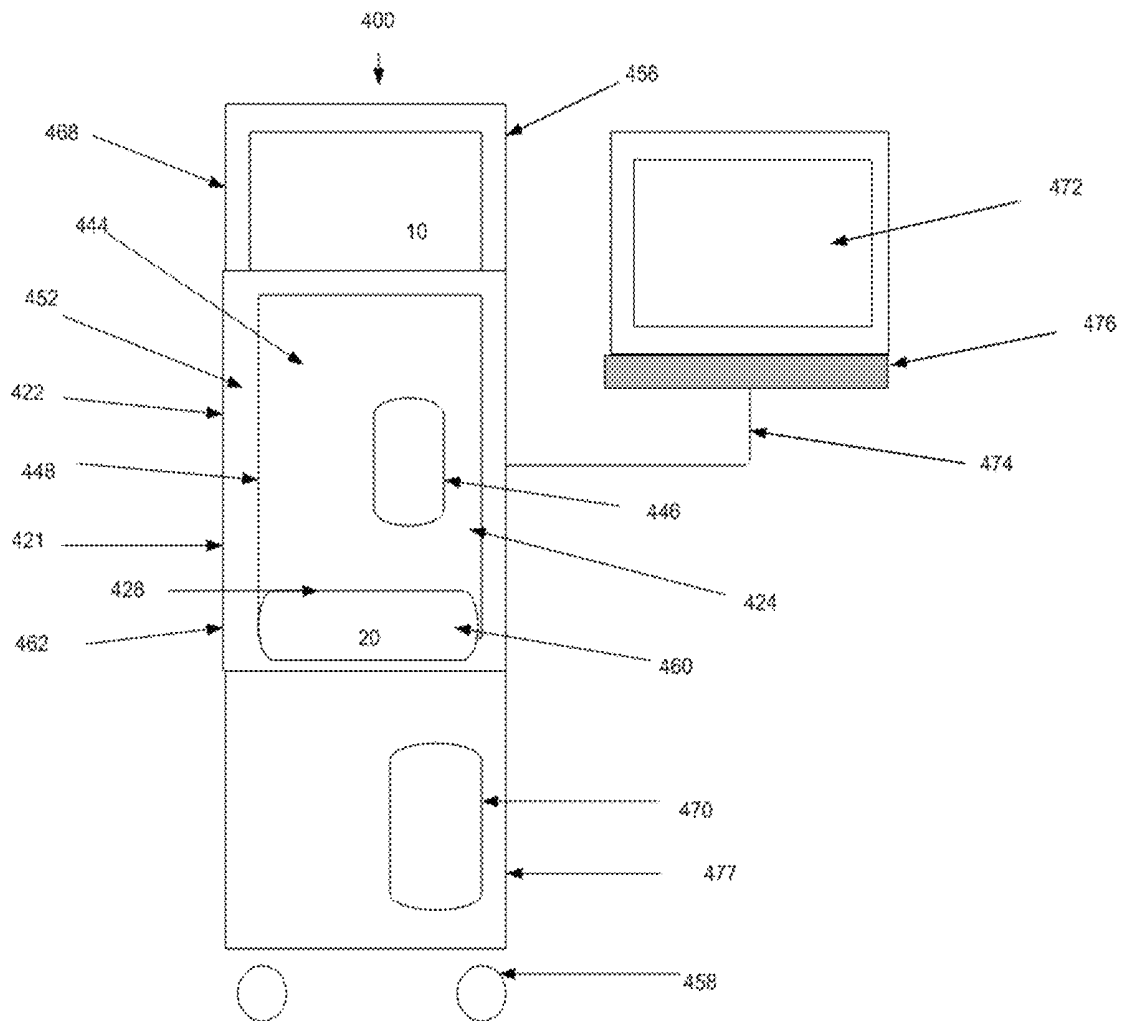
Typical Example of an X-ray Cabinet System Fig. 4
