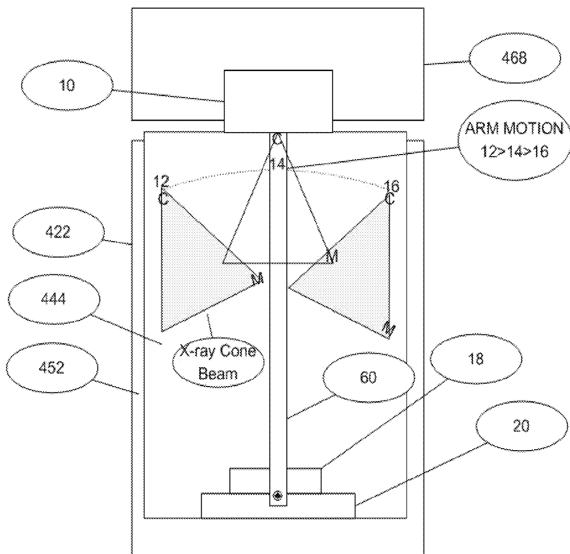
View in Sample Chamber with Door Open with X-ray source at position (14) Top Center Fig. 5
