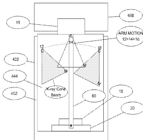
View in Sample Chamber with Door Open with X-ray source at position (14) Top Center
