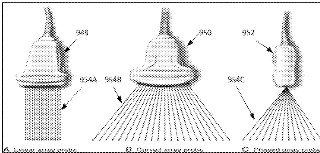
Fig. 9 – Typical Ultrasound Probes
