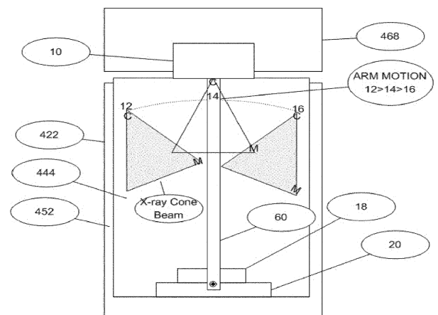
View in Sample Chamber with Door Open with X-ray source at position (14) Top Center
