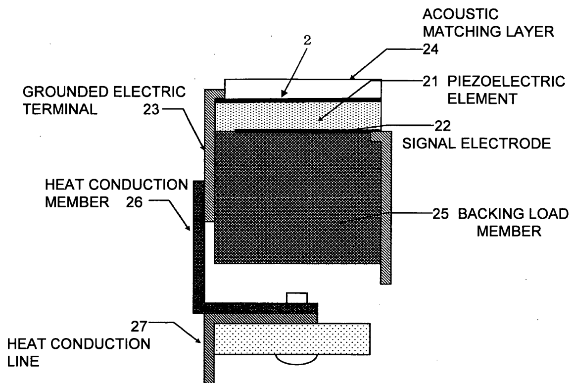
FIG. 8 PRIOR ART
