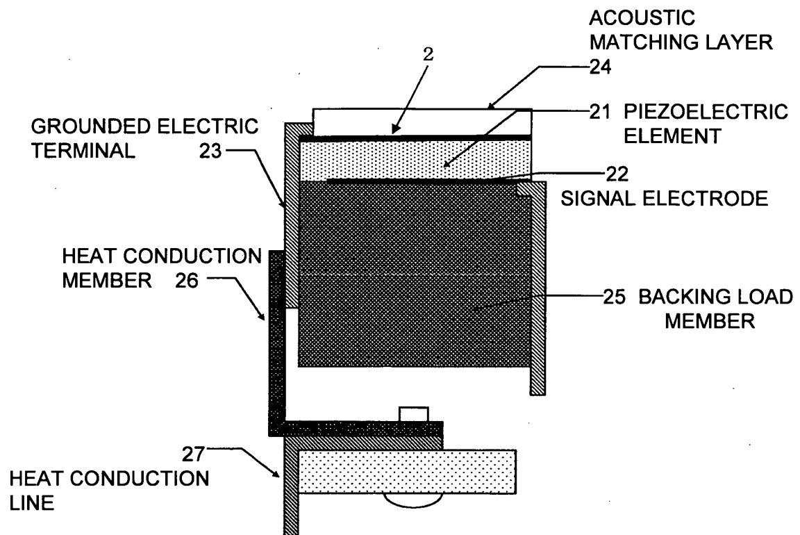
FIG. 8 PRIOR ART
