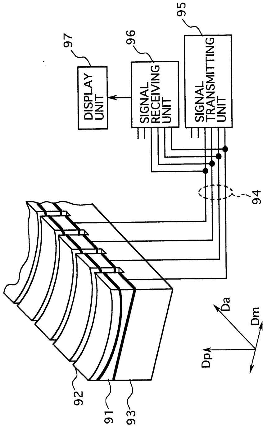
FIG.10 (PRIOR ART)
