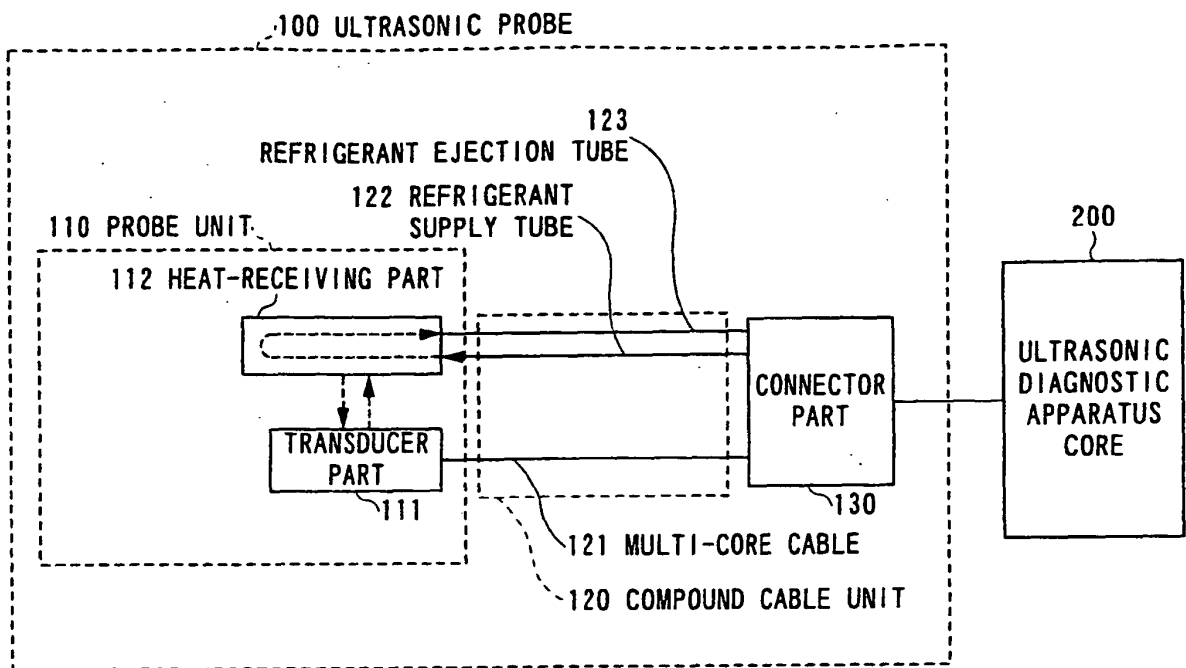
FIG. 29 PRIOR ART
