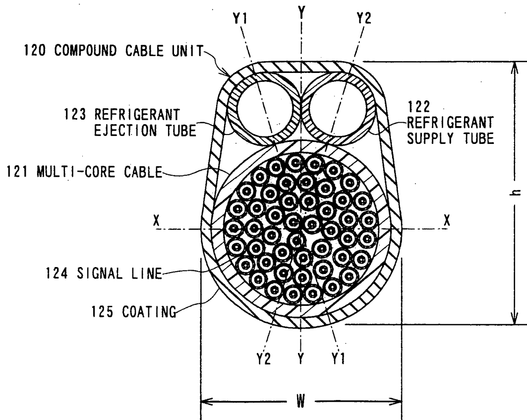
FIG. 30 PRIOR ART
