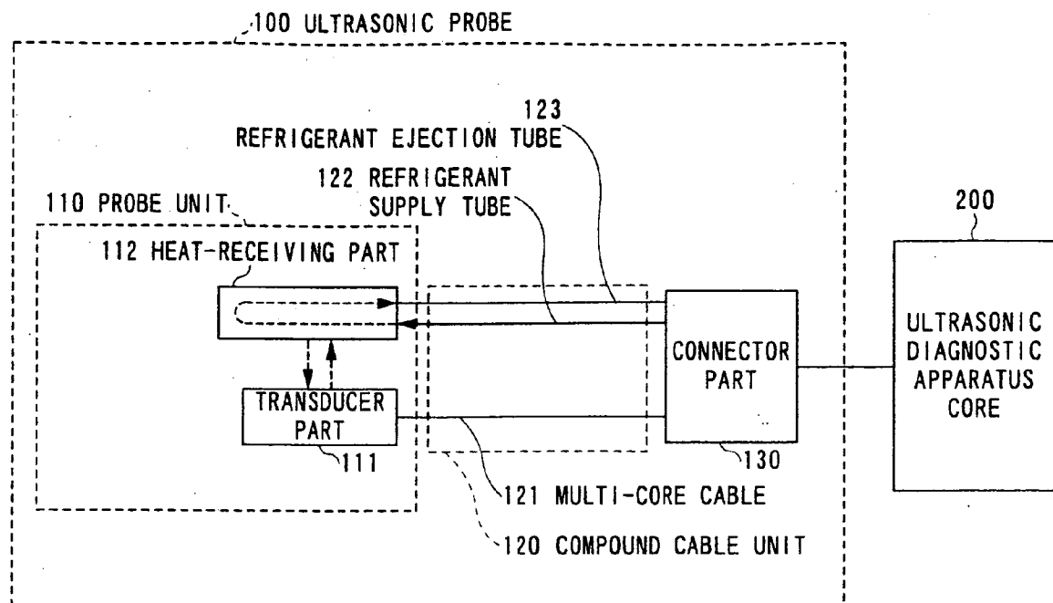
FIG. 29 PRIOR ART
