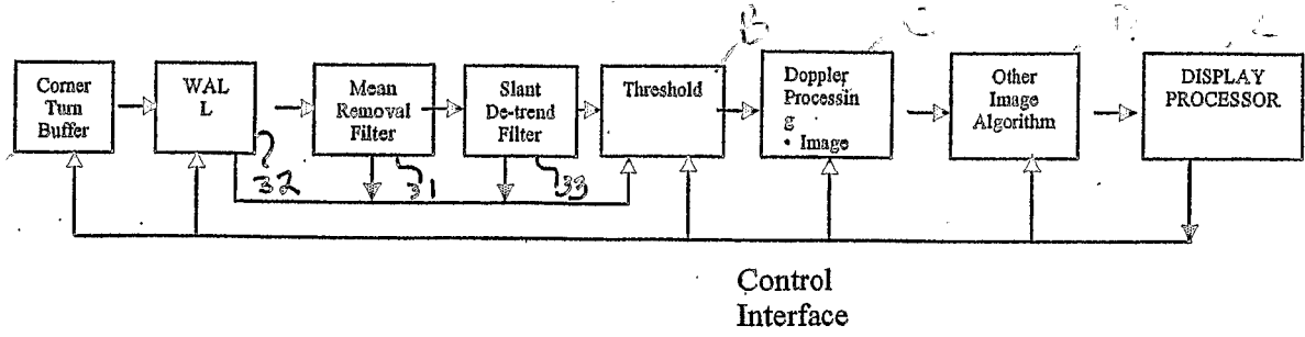
Figure 6: Improved Cascaded Filtered Ultrasound Data Flow
