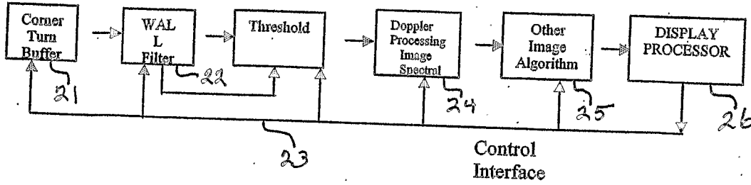
Figure 3: Ultrasound Data Flow
