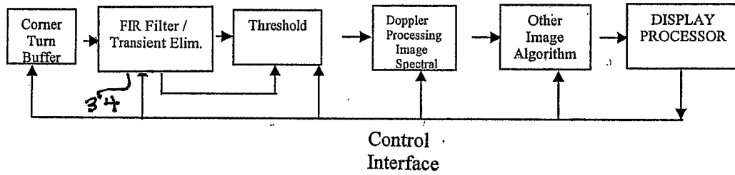
Figure 7: FIR Filter with Transient Elimination
