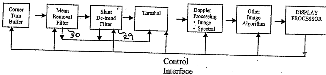
Figure 5: Alternative Ultrasound Data Flow
