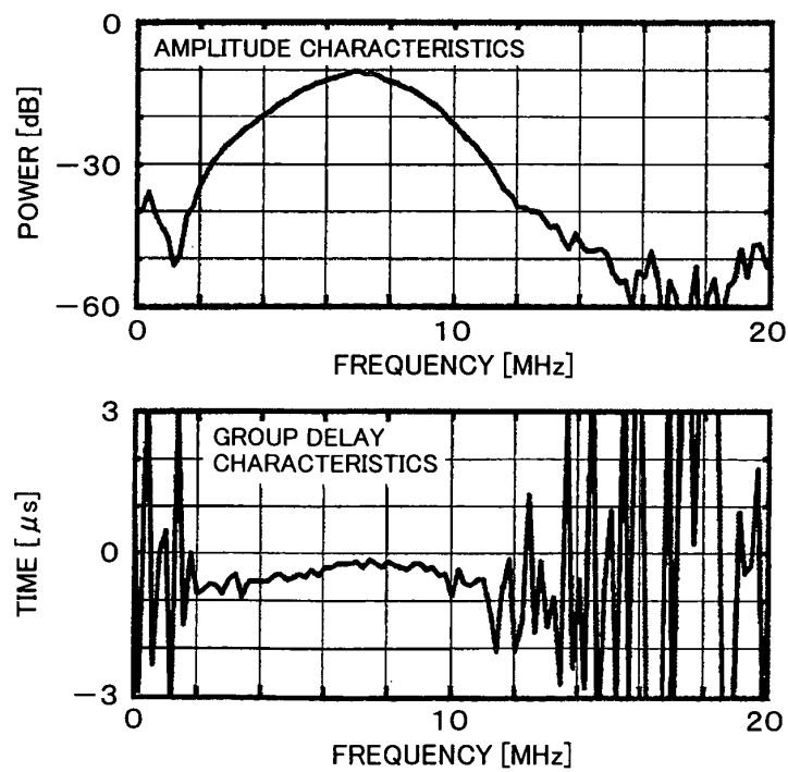
(b) FREQUENCY CHARACTERISTICS
