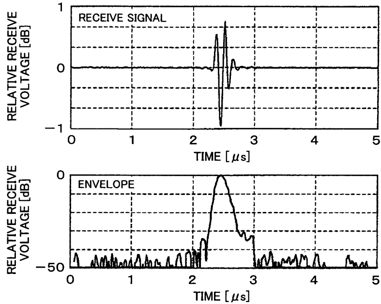
(a) PULSE CHARACTERISTICS
