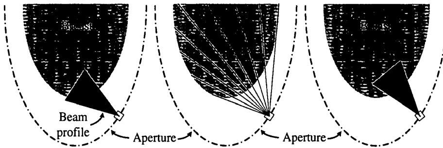
Figure 4.5: Automatic TAS normal alignment. Left: Initially the beam profile is aligned with the normal of the spheroid. Middle: Possible normals for the current TAS; each normal is evaluated in terms of maximizing the insonification with the given beam profile and incident angles. Right: Realignment of the TAS after optimization.
