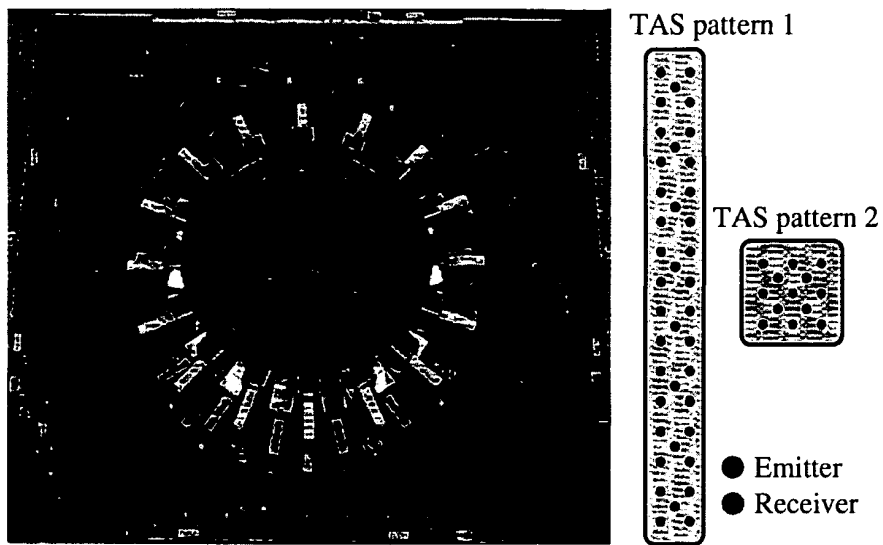
Figure 4.1: Experimental 3D USCT and different TAS patterns. The left image shows the current cylindrical USCT setup equipped with 48 TAS. A schematic of the current TAS pattern ( TAS pattern 1 ) is shown in the middle with 8 emitters and 32 receivers. An alternative TAS pattern ( TAS pattern 2 ) is shown on the right consisting of 4 emitters and 9 receivers.
