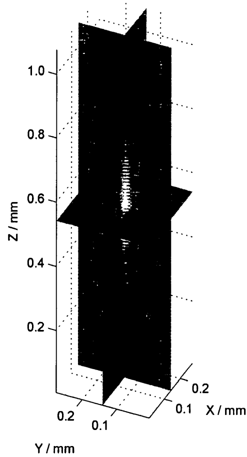
Figure 4.2: Assessment of resolution and contrast in the principal planes: Local point spread function. The resolution is evaluated by means of the shape and size of the 2D FWHM profiles (black lines) of the 3D PSF.
