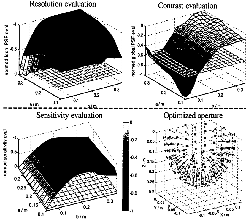
Figure 4.6: Parameter space evaluation and optimized aperture. Shown are the evaluations for each optimization criteria over the parameter space a \in [10, 35] cm and b \in [5, 35] cm at steps of 2 cm. The resulting values are mapped to the domain [-1, 0] . The plane mesh plot indicates the evaluation values for the current USCT setup in this domain. At the bottom right the optimized aperture for an equal weight of the criteria is shown ( a = 23.7 cm, b = 17.0 cm).
