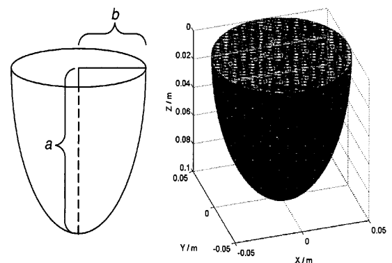
Figure 4.4: Left: Definition of a spheroid with major axis a and minor axis b . Right: Breast model with 42 positions of the point scatterers used for the analysis of resolution and contrast.
