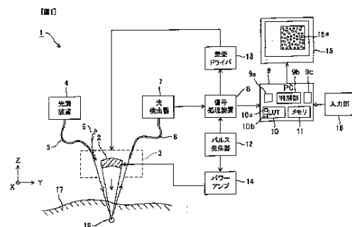
FIG. 1: 4 LIGHT SOURCE DEVICE 7 LIGHT DETECTION UNIT 8 SIGNAL PROCESSING DEVICE 9b DISCRIMINATION UNIT 11 MEMORY 12 PULSE GENERATOR 13 SCAN DRIVER 14 POWER AMPLIFIER 16 INPUT UNIT
