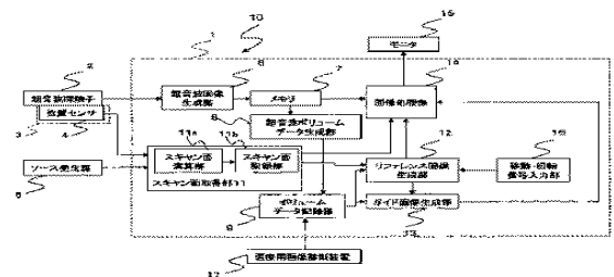
FIG. 1: 2 Ultrasound probe 4 Position sensor 5 Source generator 6 Ultrasound image generating section 7 Memory 9 Ultrasound volume data generating section 11 Scanning surface acquisition section 11a Scanning surface calculating section 11b Scanning surface recording section 12 Reference image generating section 13 Outline image generating section 14 Image processing section 15 Monitor 16 Movement and rotation signal input section 17 Medical image diagnostic device
