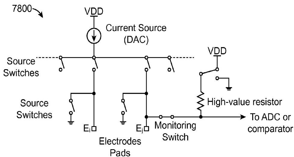
Leakage Monitoring Scheme
