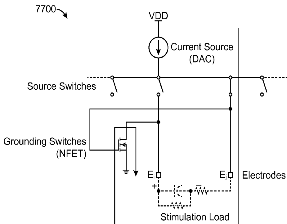
Grounding Load, Recovery Phase
