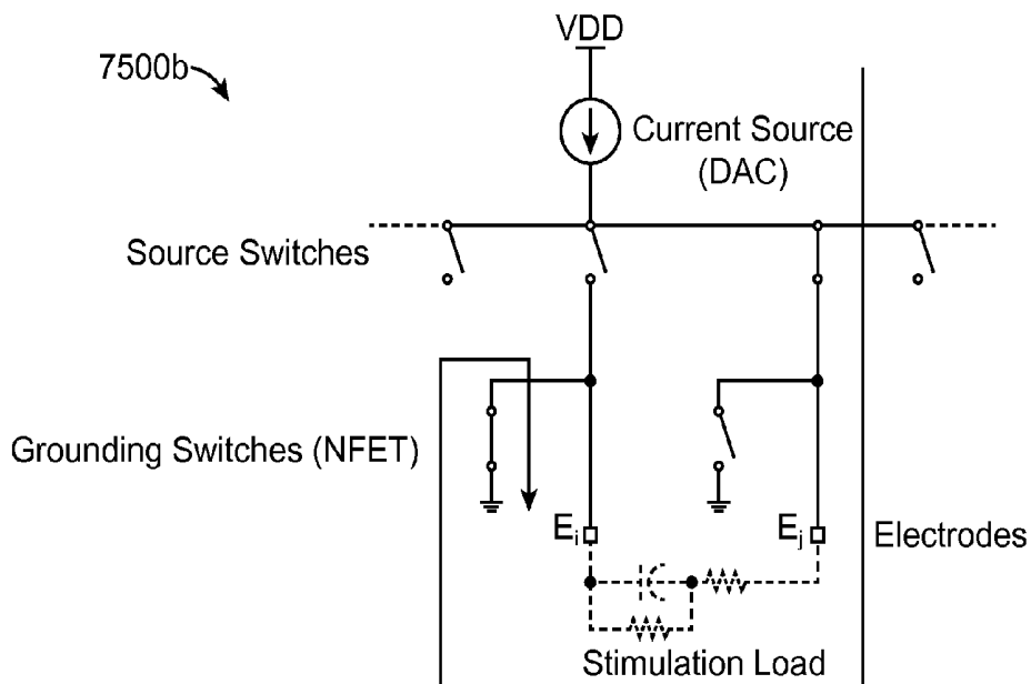
Single-channel Stimulator, Recovery Phase
