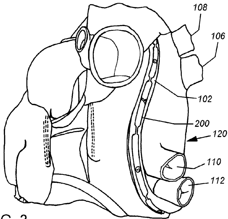
FIG. 3 (PRIOR ART)
