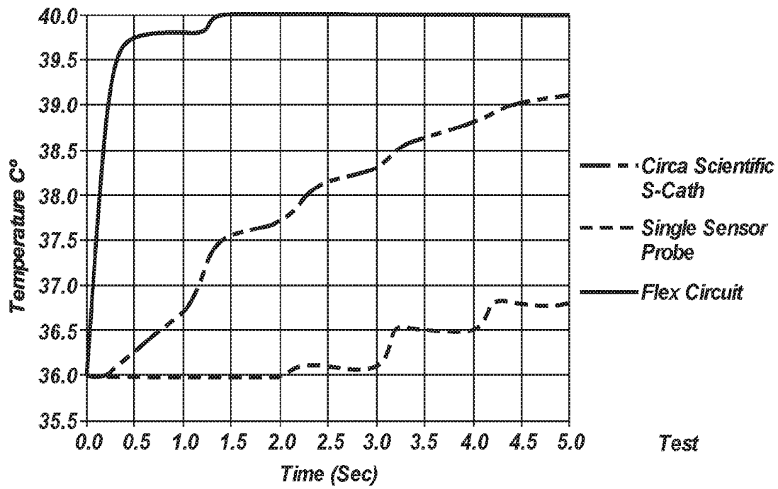
Flex Circuit Temp Probe vs. S-Cath Temp Probe vs. General Purpose Temp Probe Water Bath - 36 Degree to 40 Degree
