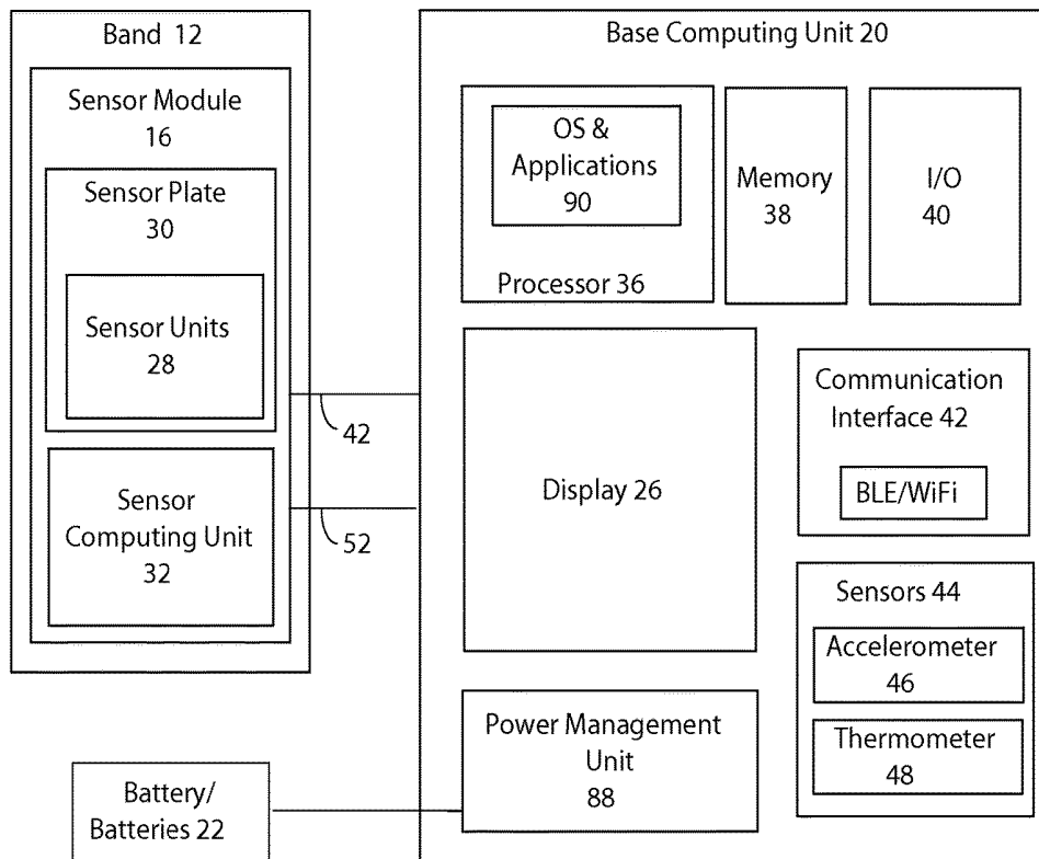
Modular Wearable Sensor Platform 10
