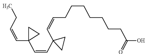
10-(1-[2-(1-But-1-enyl-cyclopropyl)-vinyl]-cyclopropyl)-dec-9-enoic acid
