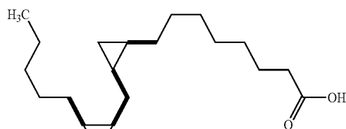
8-[2-(2-Pentyl-cyclopropylmethyl)-cyclopropyl]-octanoic acid
