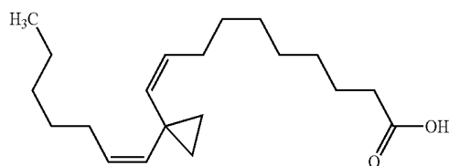
10-(1-Hept-1-enyl-cyclopropyl)-dec-9-enoic acid
