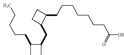
8-[2-(2-Pentyl-cyclobutylmethyl)-cyclobutyl]-octanoic acid
