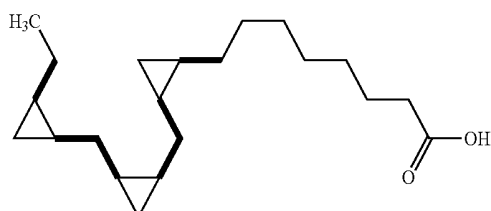
8-{2-[2-(2-Ethyl-cyclopropylmethyl)-cyclopropylmethyl]-cyclopropyl}-octanoic acid
