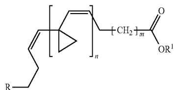
10-(1-[2-(1-But-1-enyl-cyclopropyl)-vinyl]-cyclopropyl)-dec-9-enoic acid
