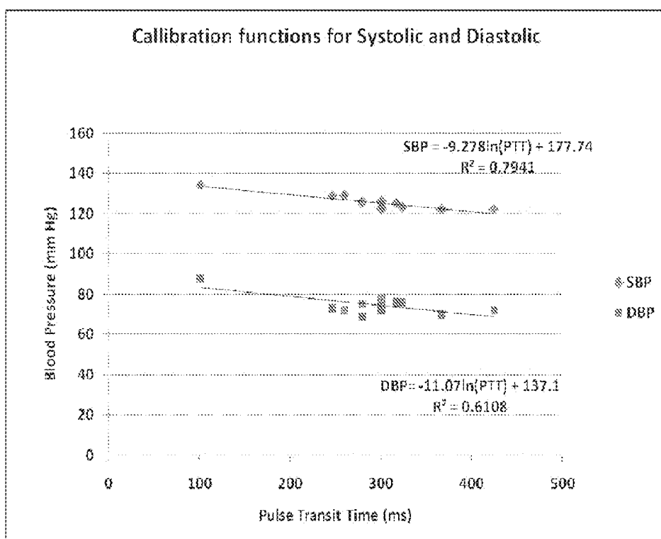
Figure. 6: Calibration curves for systolic and diastolic blood pressures versus pulse transit time.
