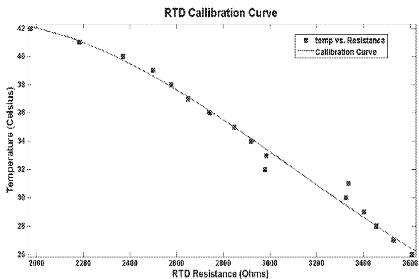
Figure 7: Resistive Temperature Detector based temperature sensor calibration curve: Temperature ( ^{\circ}\text{C} ) vs. Resistance ( \Omega )
