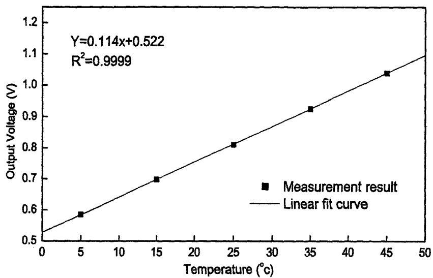
Measured V_{OUT} Versus Temperature
