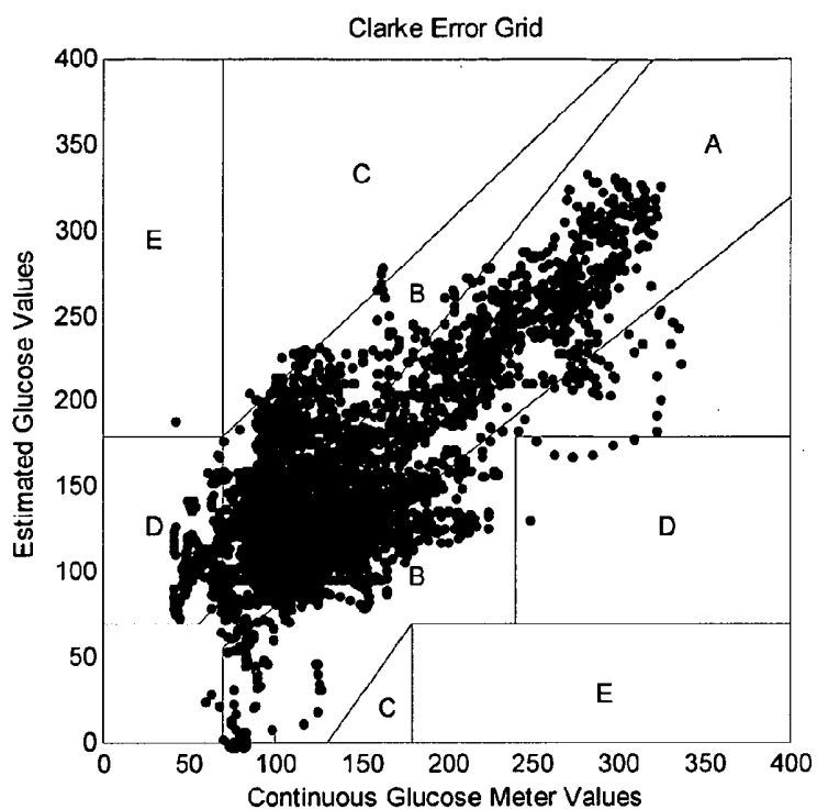
Clarke Error Grid : Estimated Glucose Vs. Continuous Glucose Meter
