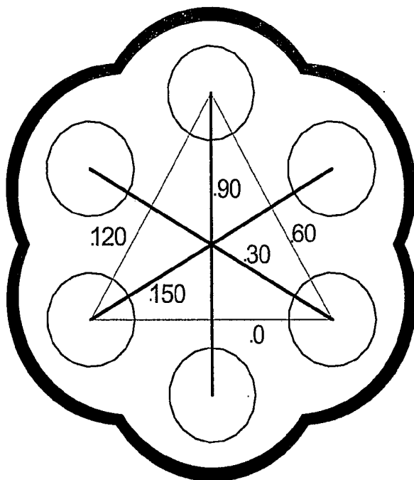
Figure 6a: ECG Views using Opposite Electrode Pairs Six Limb Lead Coverage-Vertical
