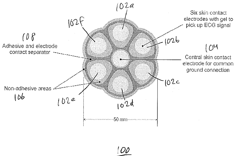
Figure 2a: One Embodiment of Multiple Electrode Scheme
