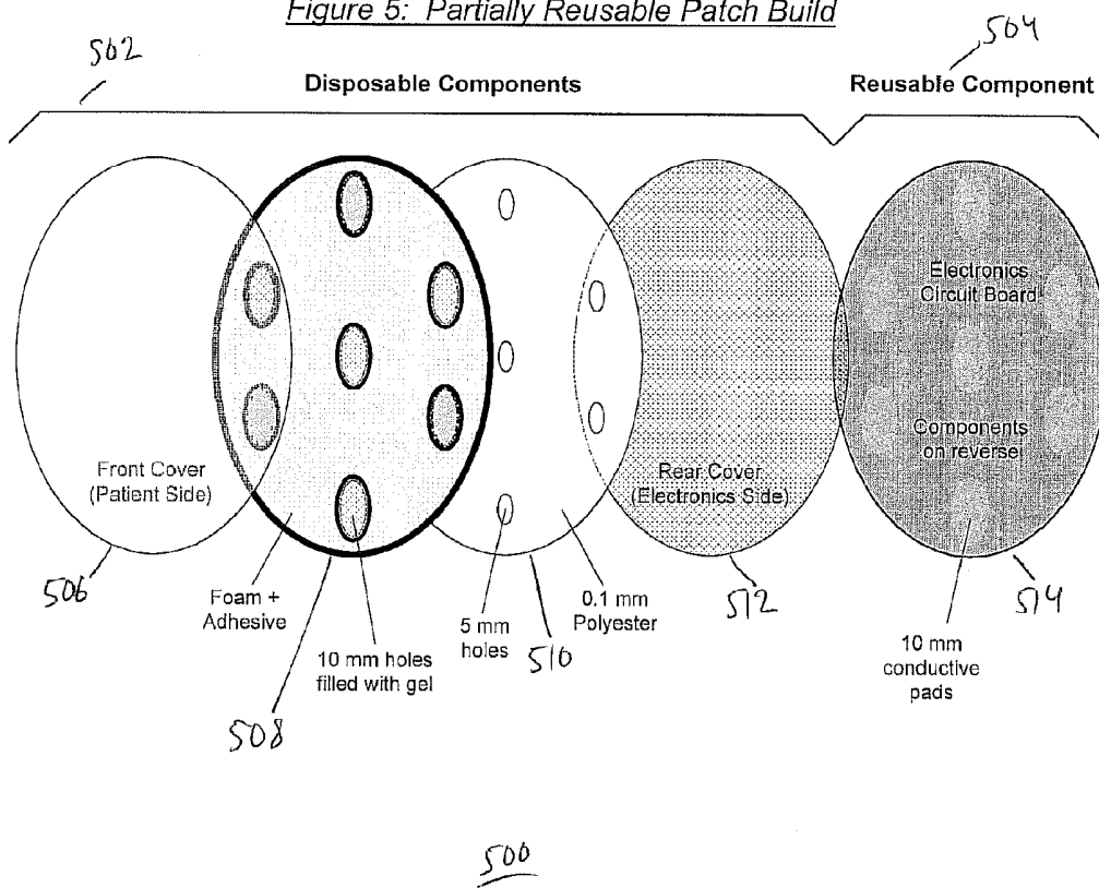
Figure 5: Partially Reusable Patch Build
