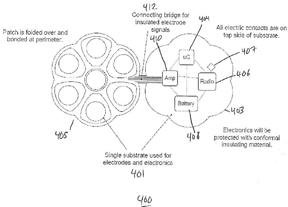
Figure 4: Fully Disposable Patch Build
