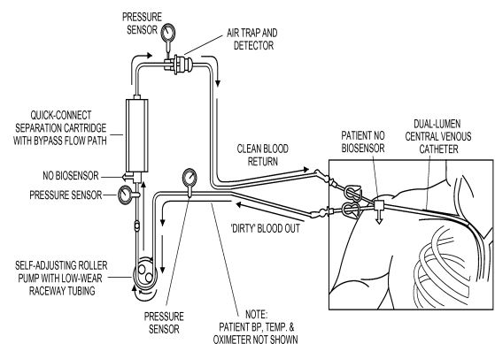
Simplified Schematic of Sepsis DLT System
