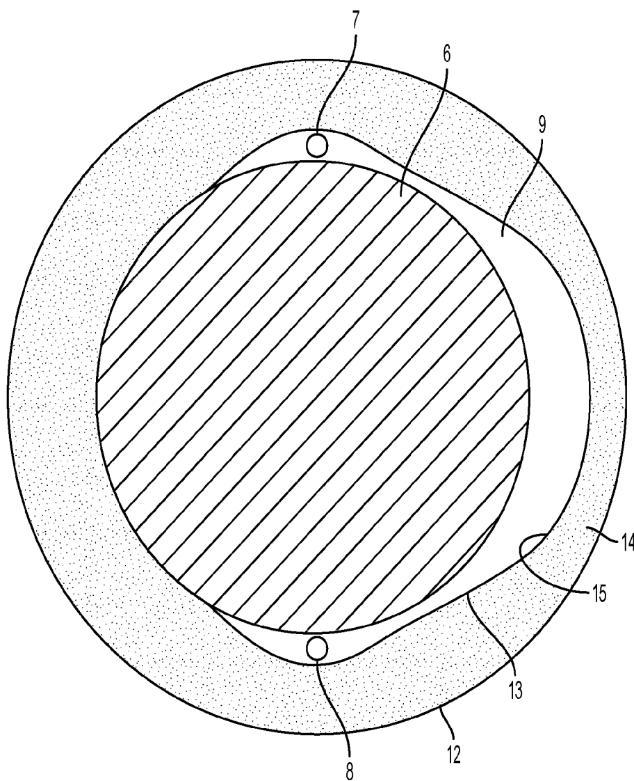
FIG. 5 PRIOR ART
