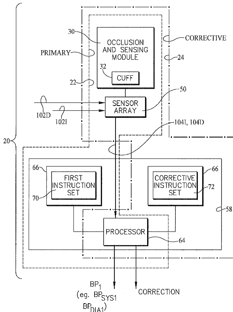
SYSTEM ARCHITECTURE OSCILLOMETRIC/OSCILLOMETRIC (0/0) - SHARED SENSOR
