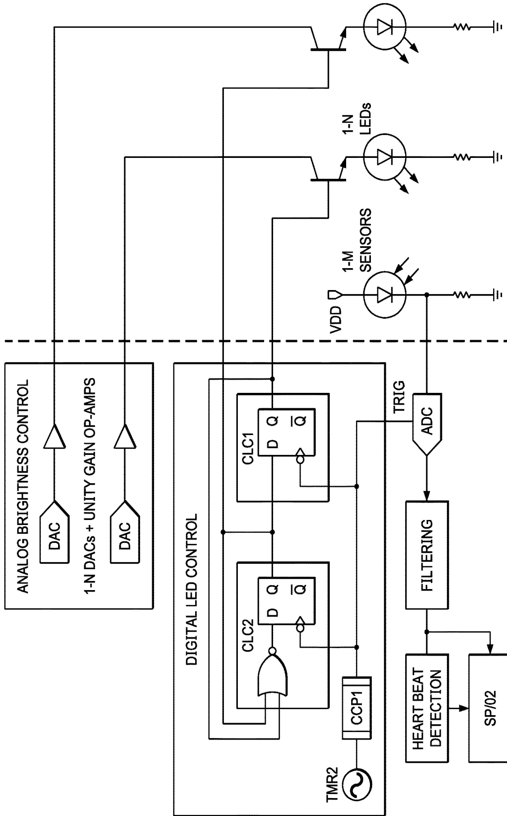
FIG. 6 (PRIOR TECHNOLOGY)
