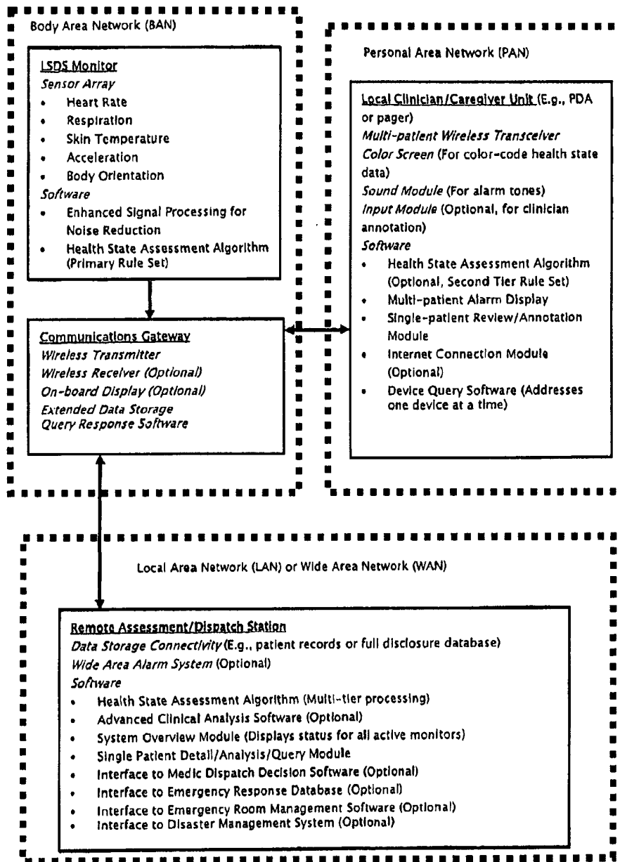
Block Diagram :Life Signs Detection System
