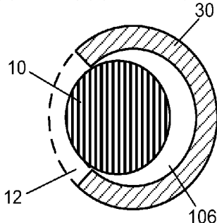
G-G CUT-THROUGH VIEW OF FIG. 1
