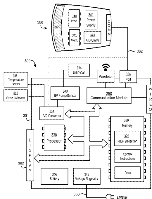
COMPONENTS OF VITAL SIGNS MONITOR
