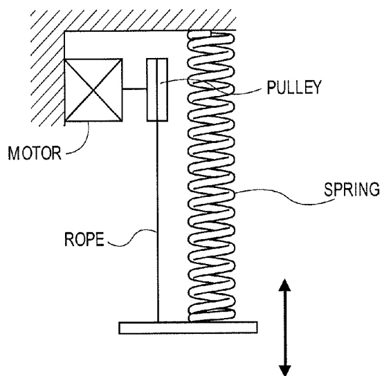
Automatic lifting mechanism
