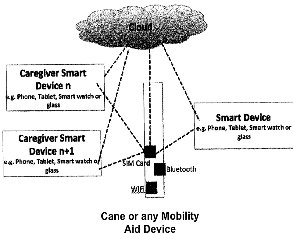
Figure 5: SIM card communication
