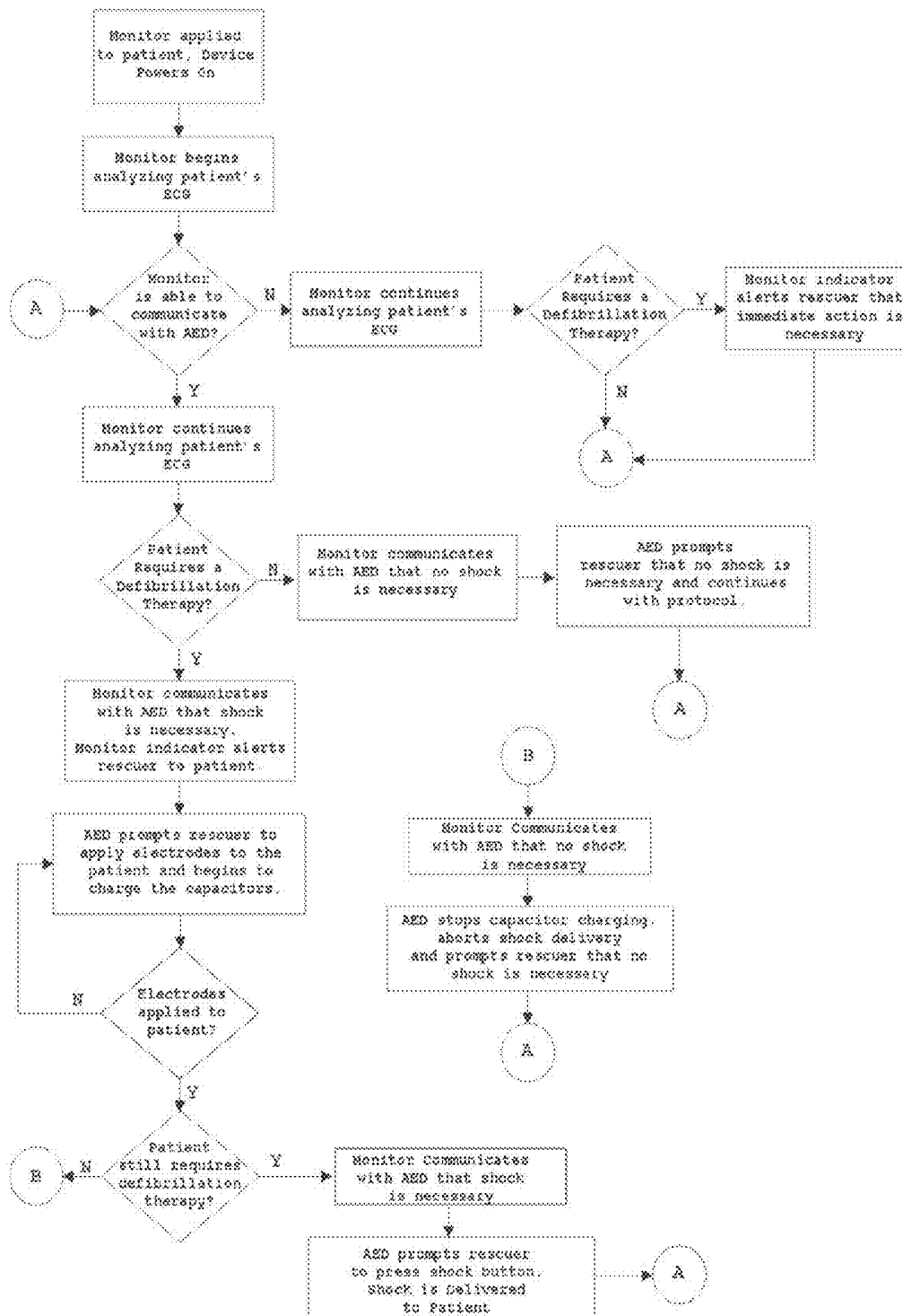
Fig.6 Method Of Monitor Communications With The AED
