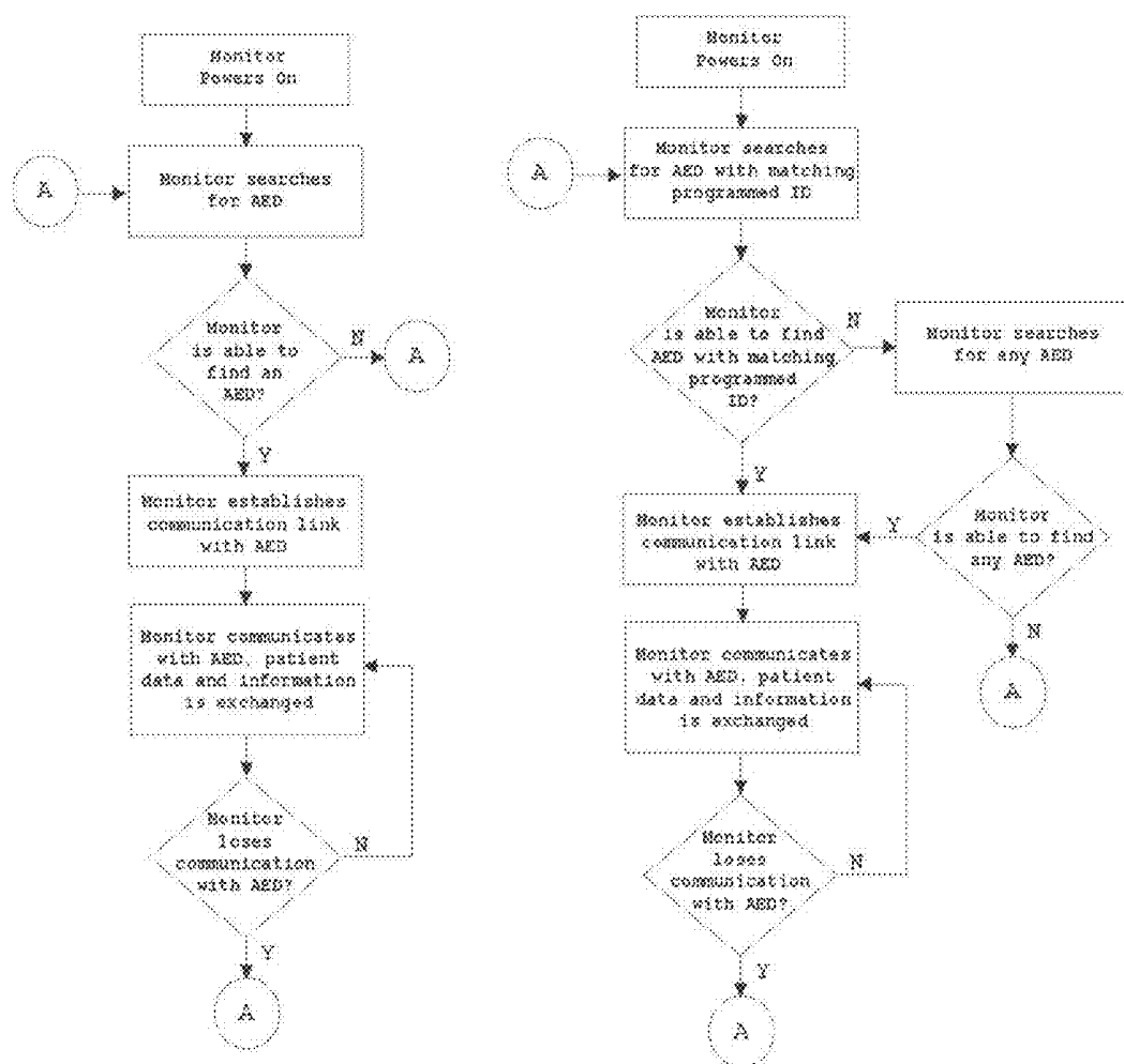
Figures 9A and 9B Methods Of Communication Link Protocol
