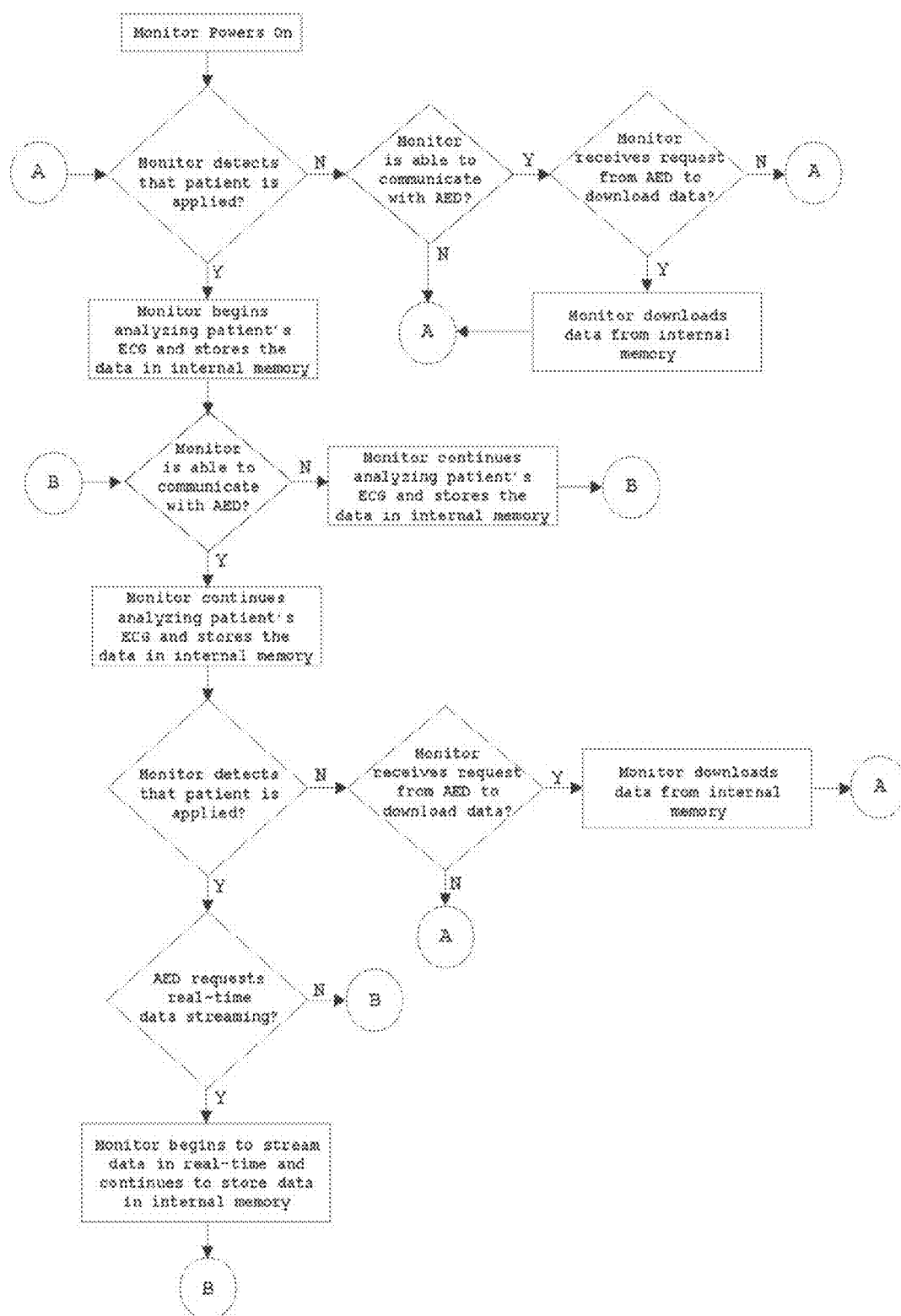
Fig.7 Method Of Monitor Data Flow To The AED
