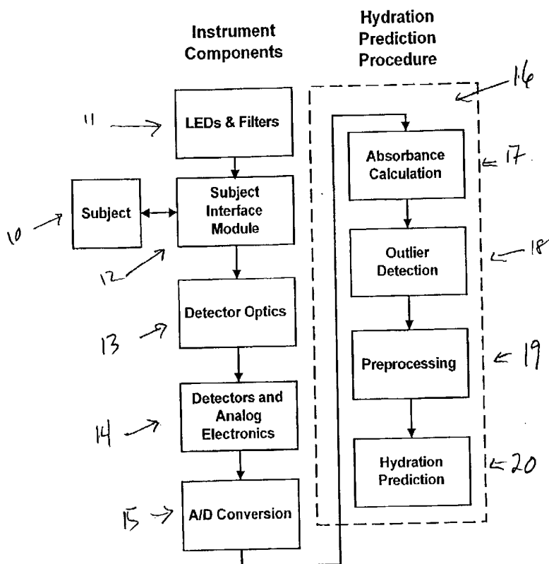
Hydration Prediction System -- Block diagram of the instrument and hydration prediction procedure.
