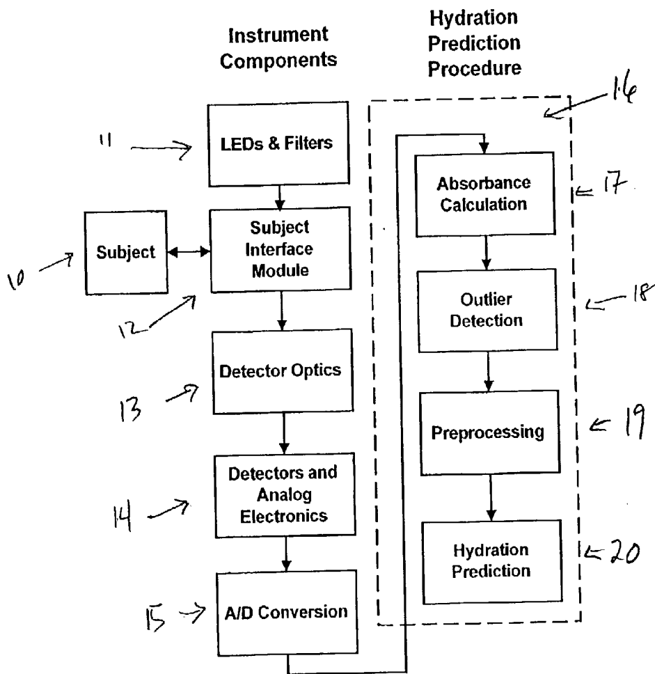
Figure 1. Hydration Prediction System -- Block diagram of the instrument and hydration prediction procedure.
