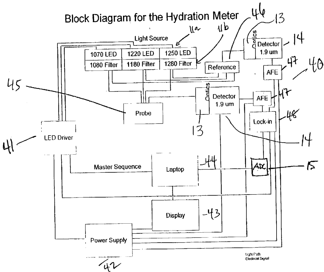
Figure 3. Block Diagram for Hydration Meter.
