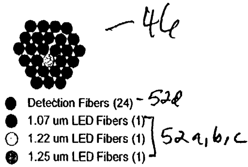
Figure 6 Reference Probe Head Fiber Optic Arrangement.
