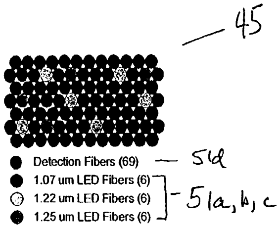
Figure 5 Sample Probe Head Optimal Fiber Optic Arrangement.
