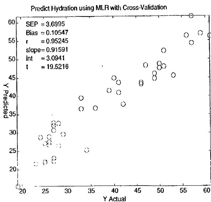
Figure 7 Prediction of Hydration of the Experimental Data using MLR with Cross-Validation
