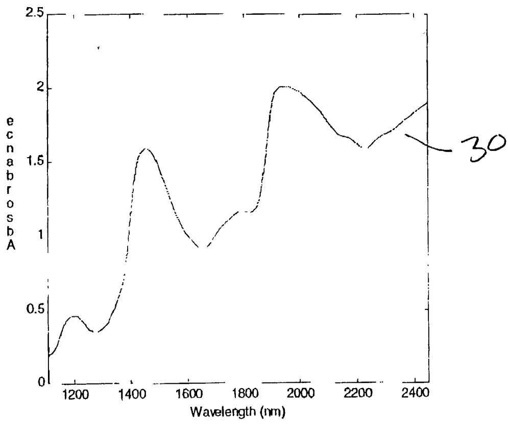
Figure 2. Typical noninvasive absorbance spectrum.
