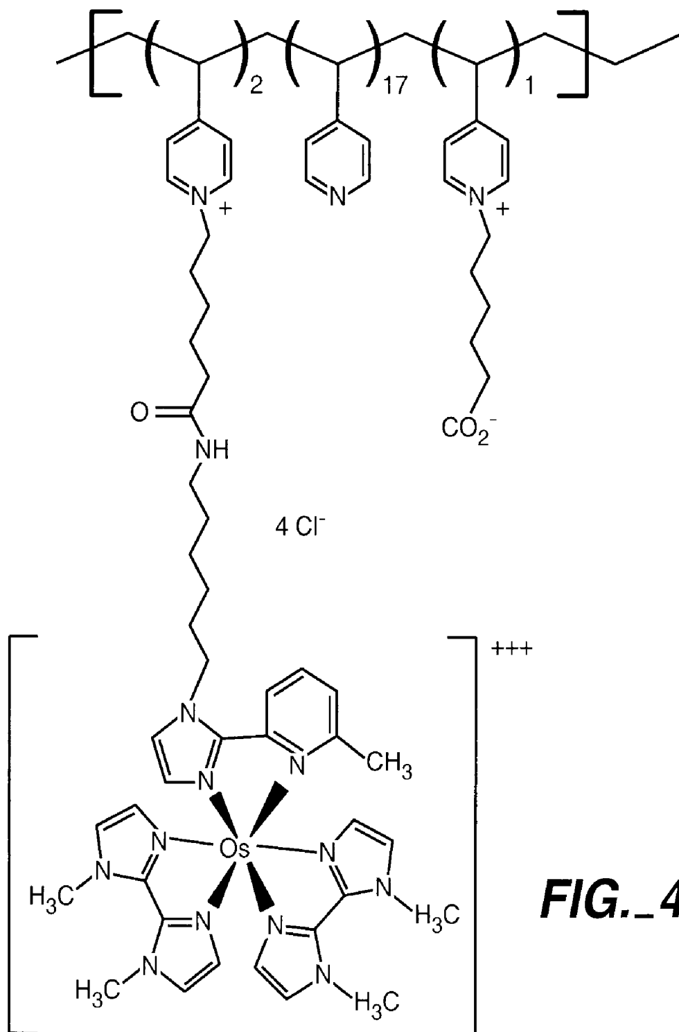
Structure of Redox Polymer 316
