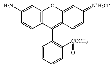
Structure A: Rhodamine 123 (Rh-123)
