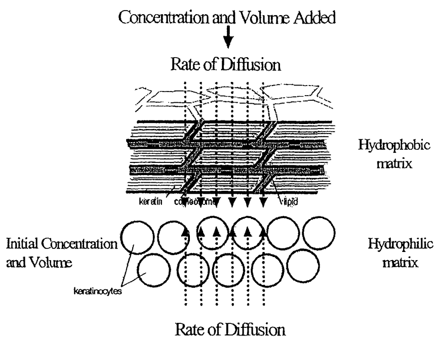
Scheme 4. In Vivo Calibration Issues
