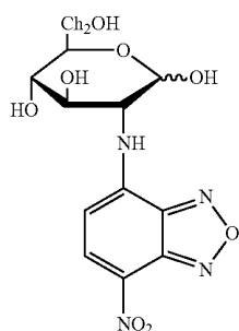
Structure E: 2-(N-(7-nitrobenz-2-oxa-1,3-diazol-4-yl)amino)-2-deoxyglucose (2-NBDG)
