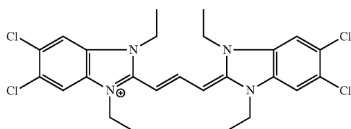
Structure D: T-3168
