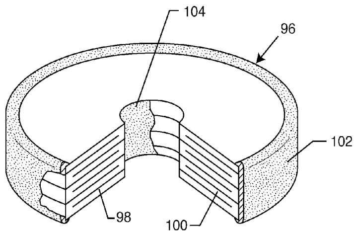
FIG. 21 PRIOR ART
