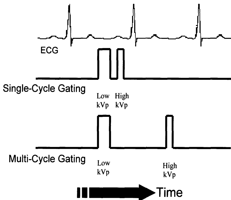
Figure 4: A schematic illustration of the timing of the two exposures in a gated dual-energy procedure. The Exposure times are shown relative to the cardiac cycle for both the single-cycle and multi-cycle gating modes.
