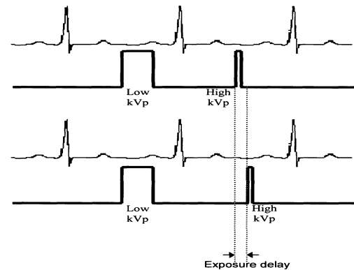
A schematic illustration of the two different approaches to timing the two exposures in an ECG-gated dual-energy procedure.
