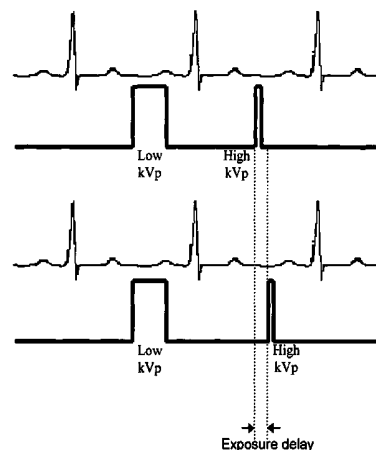
A schematic illustration of the two different approaches to timing the two exposures in an ECG-gated dual-energy procedure.
