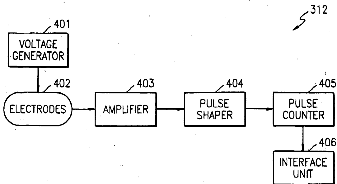
FIG. 4 (PRIOR ART)
