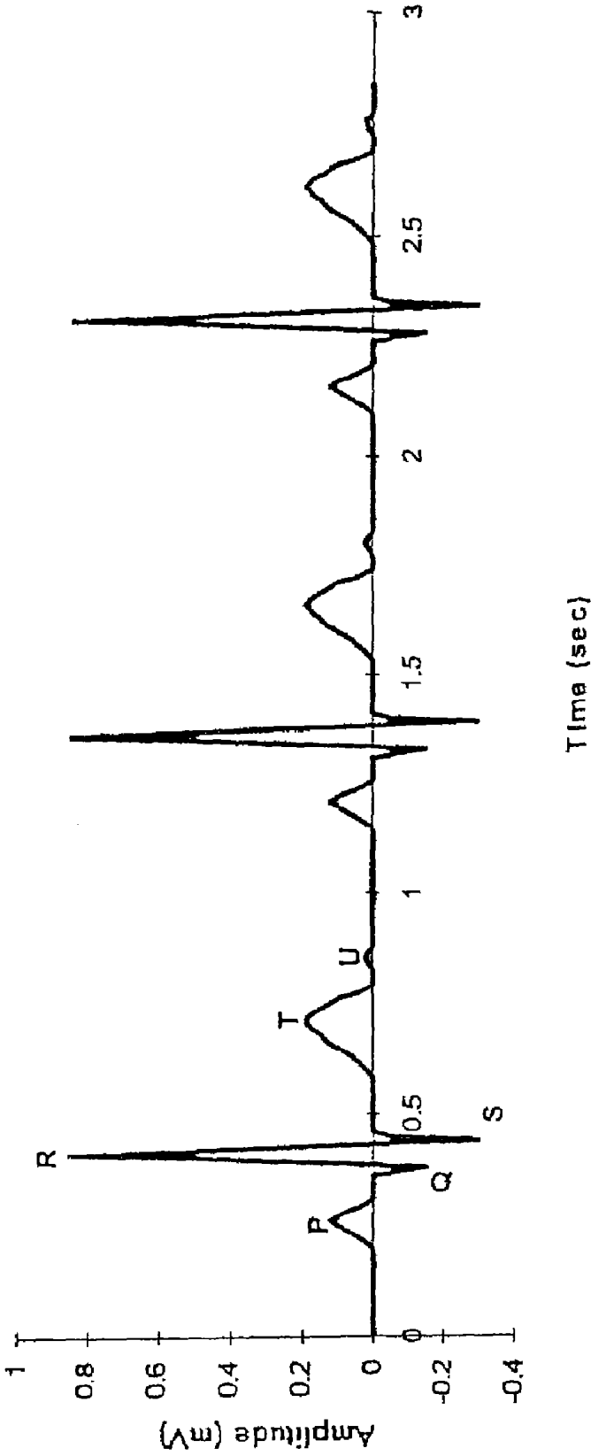
ECG Trace : Normal Supraventricular Rhythm
