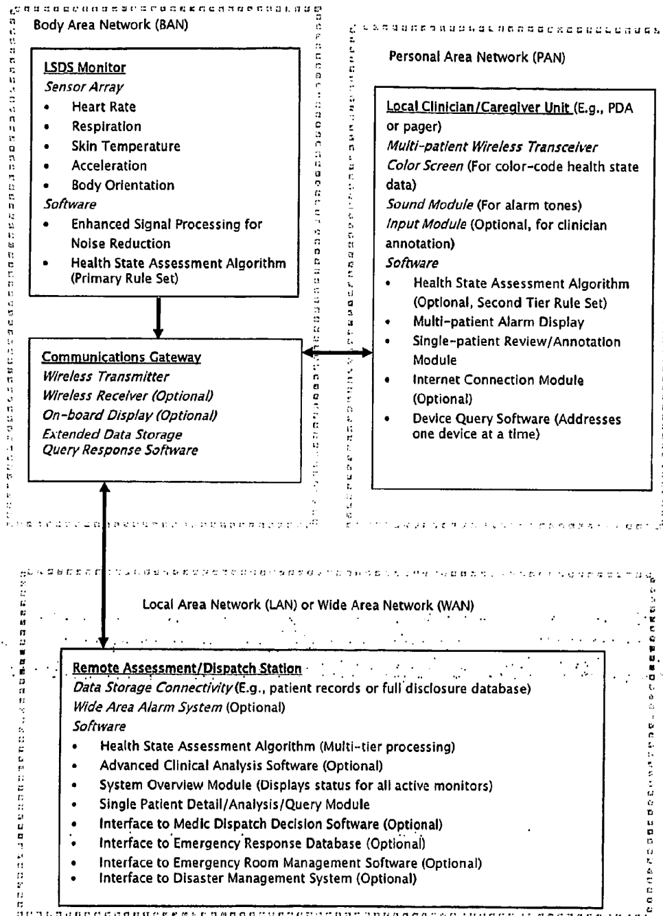
Figure 48 - Block Diagram :Life Signs Detection System
