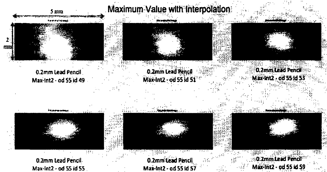
Figure 4: C-scan images of lead pencil exposed by 2mm laser beam
