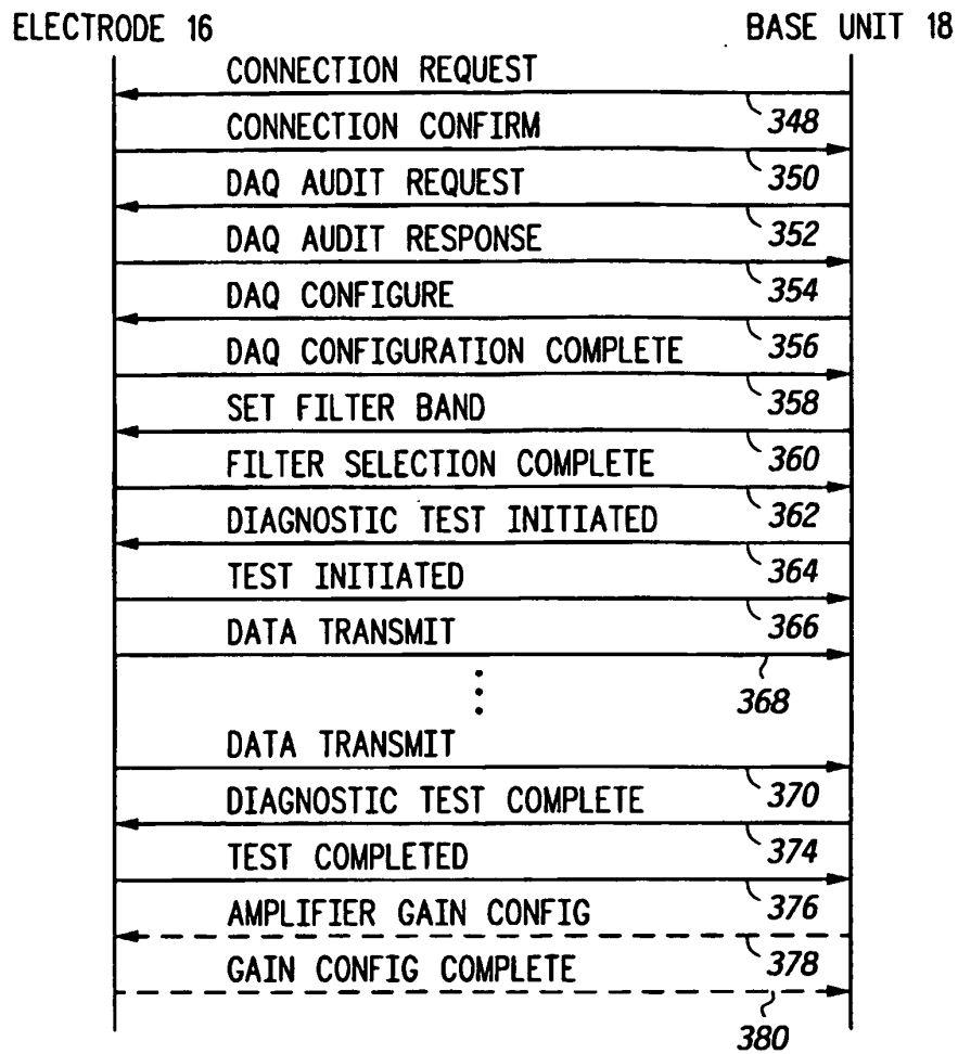
FIG.29 MONITORING CONFIGURE SCENARIO
