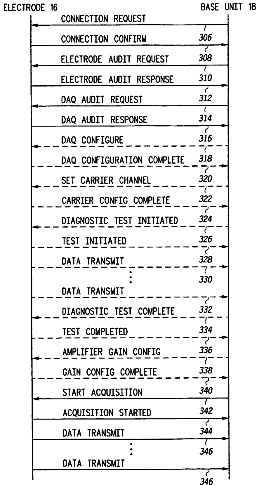
FIG.28 SIGNAL LOSS/CHANNEL ERROR RECOVERY SCENARIO
