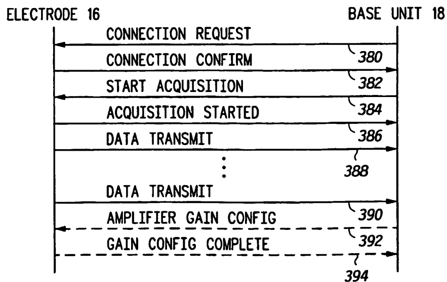
FIG.30 MONITORING START SCENARIO
