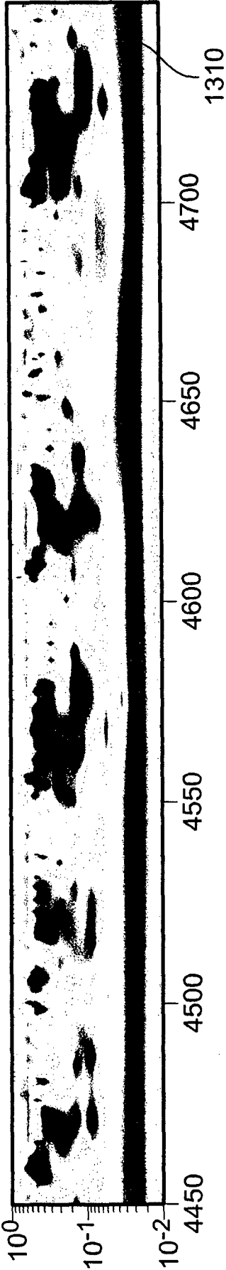
Scalogram R
