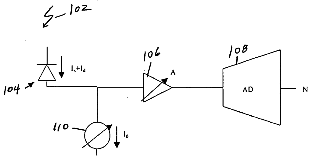
Figure 13. Diagram of SpO2 Measuring Circuit
