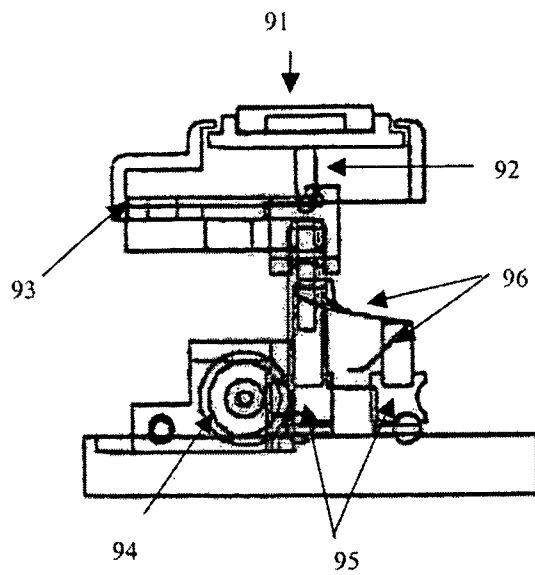
Figure 12. Illustration of SpO2 active pressure device.
