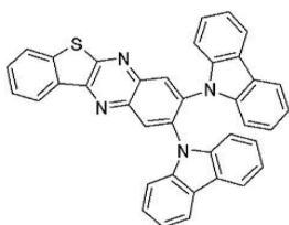
compound 2
