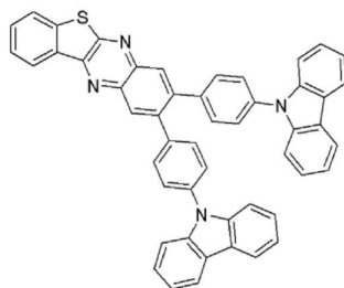
compound 4
