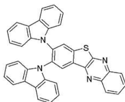
compound 4
