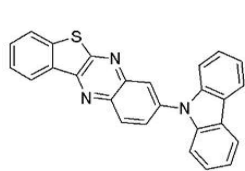
compound 1
