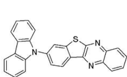
compound 3
