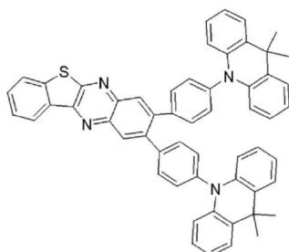
compound 12
