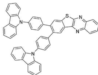
compound 8
