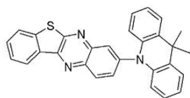
compound 9
