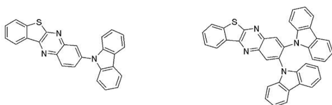
compound 1
