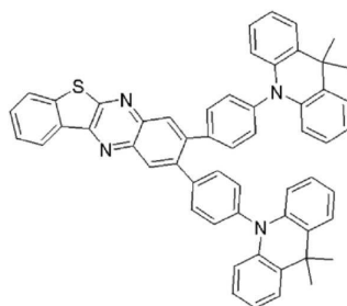
compound 12
