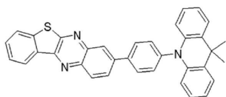
compound 11
