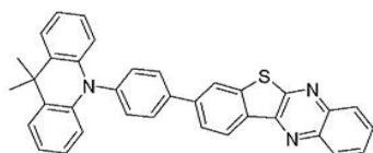
compound 15
