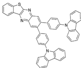
compound 4
