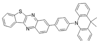
compound 11
