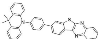
compound 15
