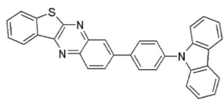
compound 3
