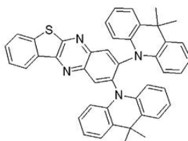
compound 10
