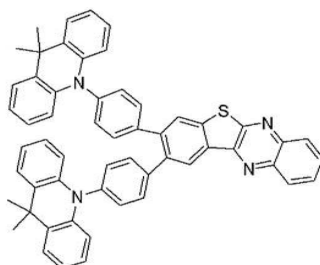
compound 16
