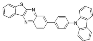
compound 3
