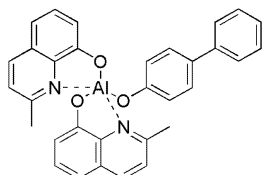
BAIq
