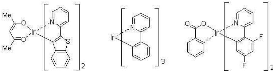
(acac)Ir(btp) 2 Ir(ppy) 3 Firpic
