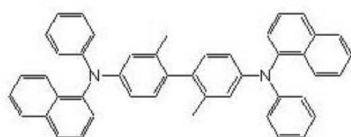
α-NPD
