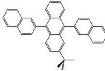
TBADN
