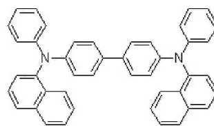
NPB
