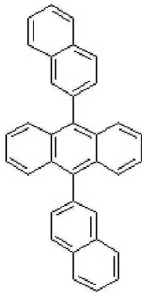
DNA
