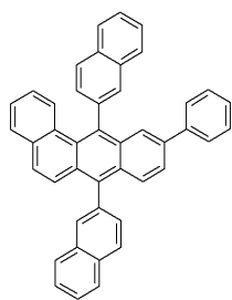
DNPBA
