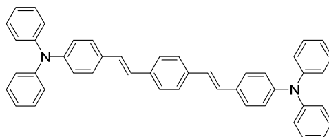
DSA-Ph
