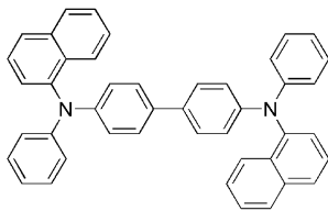
NPB
