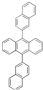
DNA
